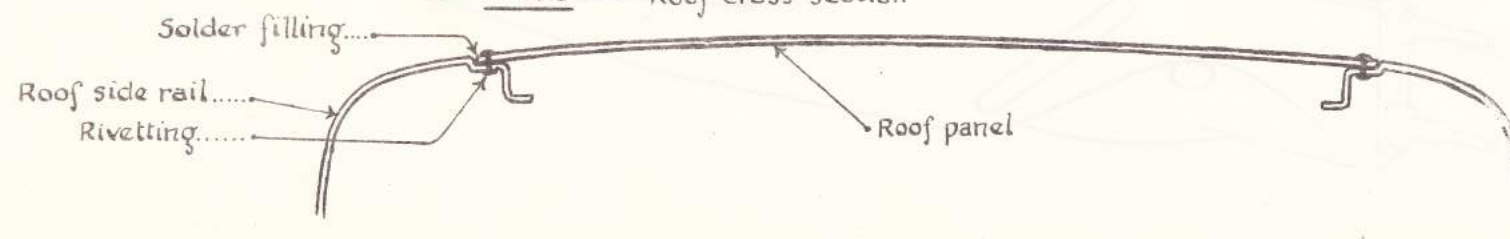
— Fig. 2. — Roof cross section
