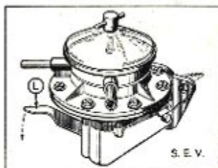
Fig. 3. — POMPES A ESSENCE.
